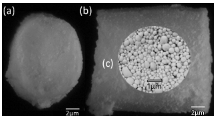
Figure 1. Europium-yttria rod obtained by bio-prototyping and sintering at 1600^{\circ}\text{C} for 4h. Optical images of (a) superior view and (b) lateral view; (c) microstructure of rod surface by SEM.
